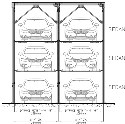
Model VSS-PH3-L
