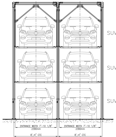
Model VSS-PH3-S
