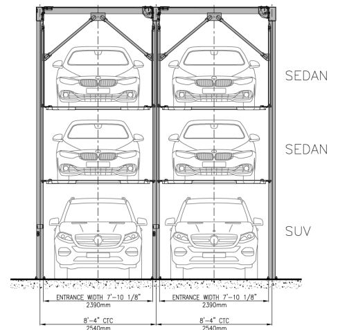
Model VSS-PH3-SL
